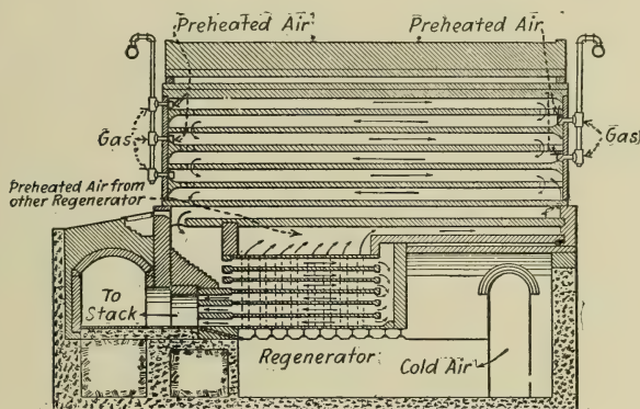
Fig. 89.—Semet-Solvay Coke-oven.
